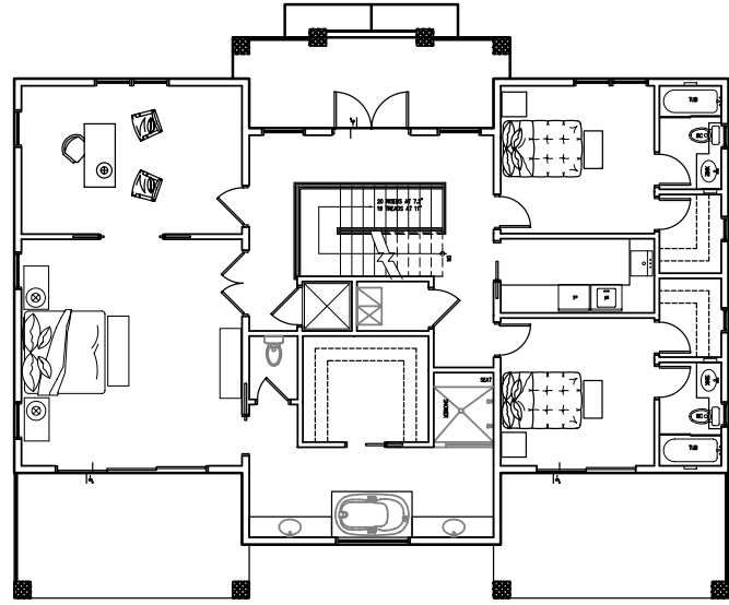
THIRD FLOOR PLAN 1/8"=1'-0"
