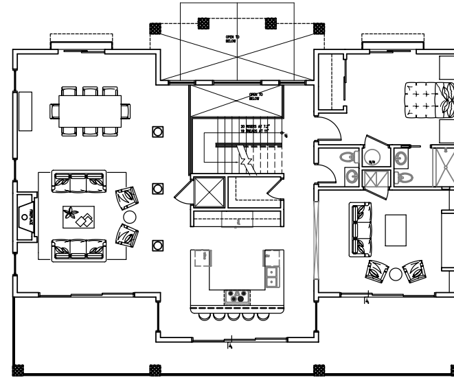
SECOND FLOOR PLAN 1/8"=1'-0"
